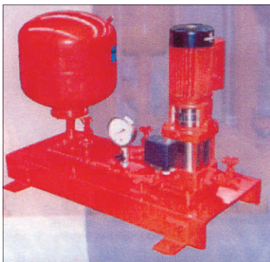
Pumps complete with pressure switch & pressure tank on a baseplate
